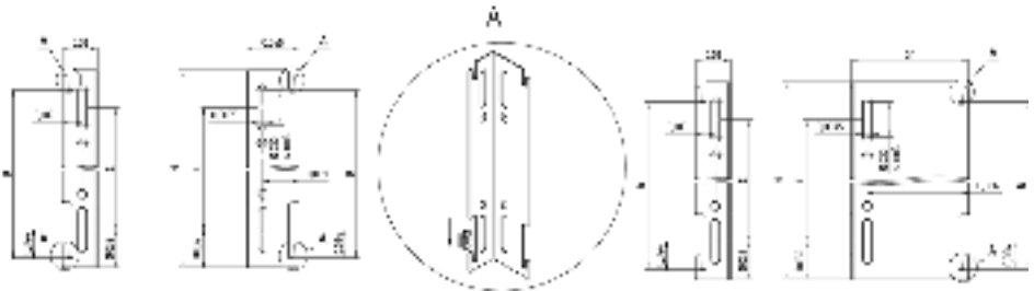
Габариты для радиаторов с полкой к стене (для радиаторов 11, 12, 13, 14, 15, 16, 17, 18, 19, 20, 21, 22, 23, 24, 25, 26, 27, 28, 29, 30)
